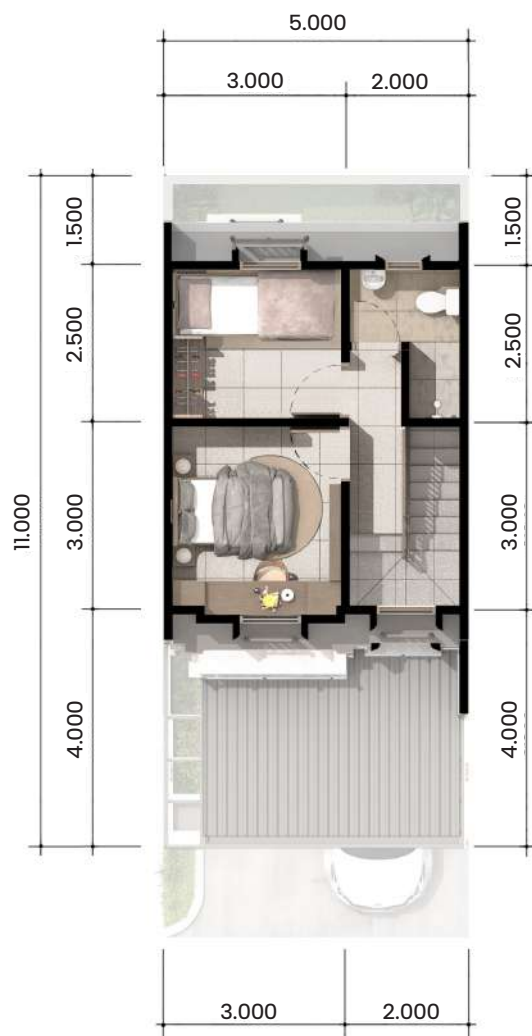
FLOOR 3
